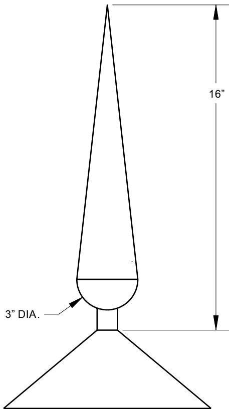
ELEVATION VIEW
