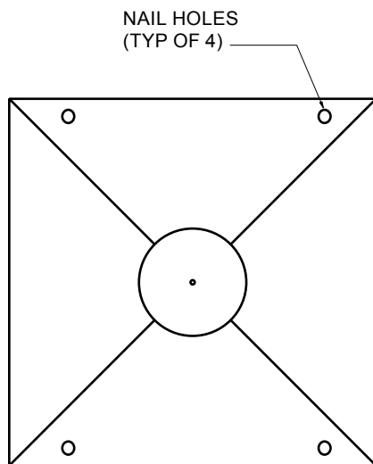
PLAN VIEW
