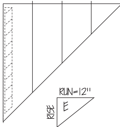
SECTION VIEW
