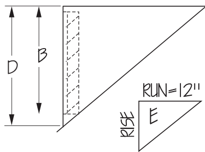
SECTION VIEW
