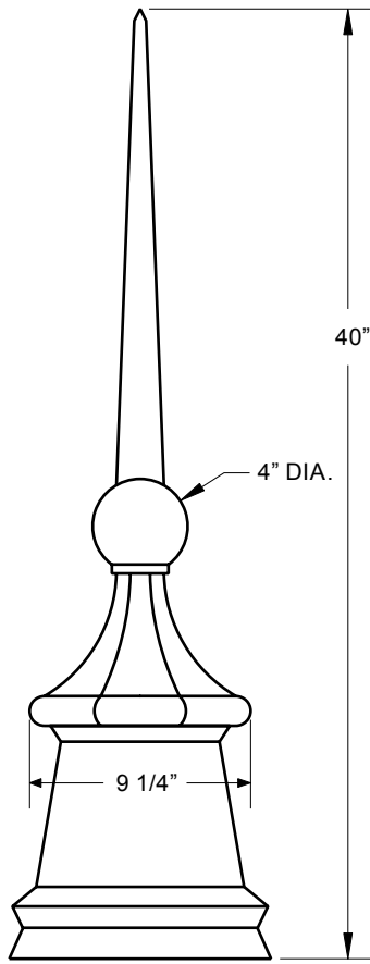
ELEVATION VIEW
